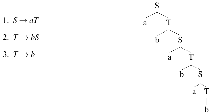
Figure 1: A regular grammar for generating (ab)^n , along with a tree diagram for the string ababab generated by the grammar.
