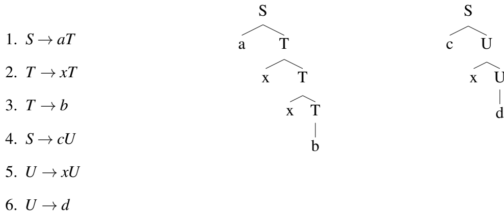
Figure 3: A regular grammar which generates a stringset which is not strictly local, and tree diagrams for two strings that it generates.
