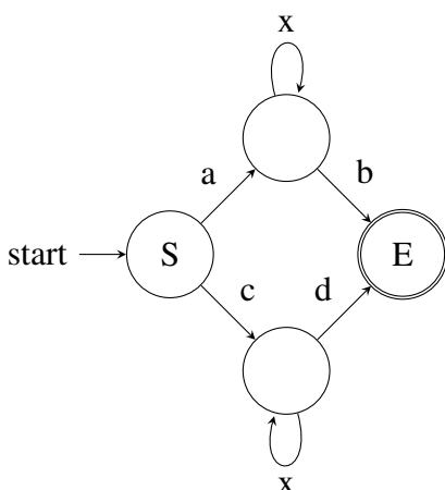
Figure 4: Finite-state automaton for recognizing the stringset ax^*b \mid cx^*d .
