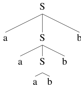
Figure 2: A context-free grammar for generating a^n b^n , and a tree diagram for aaabbb .
