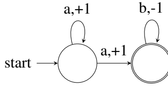
Figure 5: A counter automaton for recognizing a^n b^n
