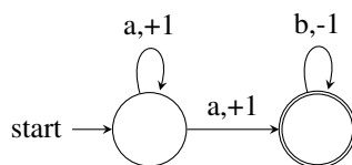
Figure 5: A counter automaton for recognizing a^n b^n
