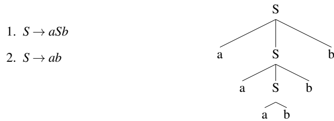
Figure 2: A context-free grammar for generating a^n b^n , and a tree diagram for aaabbb .
